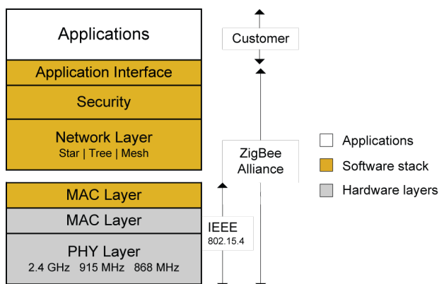
Figure 1.2. Zigbee Architecture
